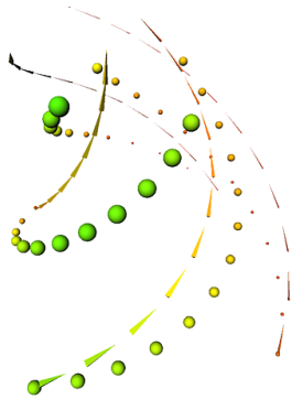
Fig. 3. Colored streak balls and tetrahedra in a vortex flow given on a sparse grid.
