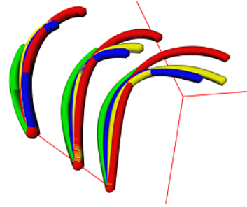
Fig. 4. Streak tubes in a cavity flow; the red tubes are computed on a full grid of level 7, the other tubes are created on sparse grids of level 7 (yellow), 5 (blue), and 3 (green).
